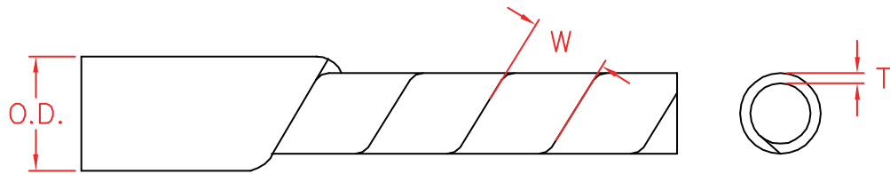
O.D. AS PRODUCTION ( BEFORE CUT IN LENGTH )
